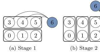
Fig. 7. Hypercube view of prime merging with seven processes.
